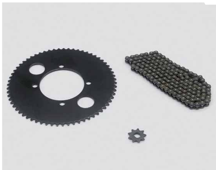
KIT TRANSMISSION (COURONNE 65T, PIGNON 9T, CHÂÎNE 140T) TRANSMISSION KIT (65T SPROCKET, 9T FRONT SPROCKET, 140T CHAIN)
